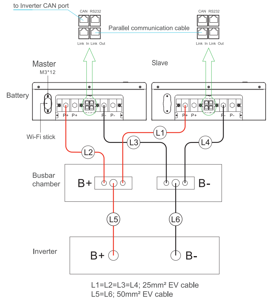
Scheme Two (Inverter Power > 5KW)
