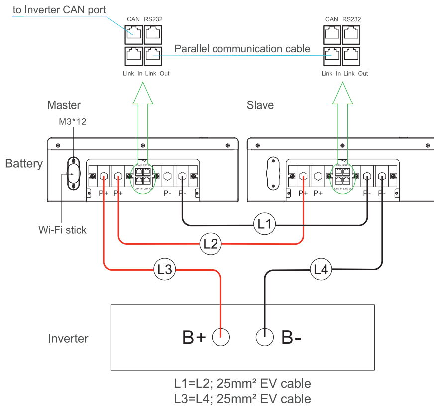
Scheme One (Inverter Power \leq 5\text{KW} )
